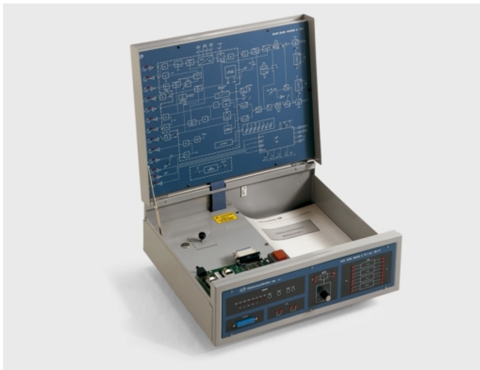
BASE BAND MODEM mod. BM/EV
