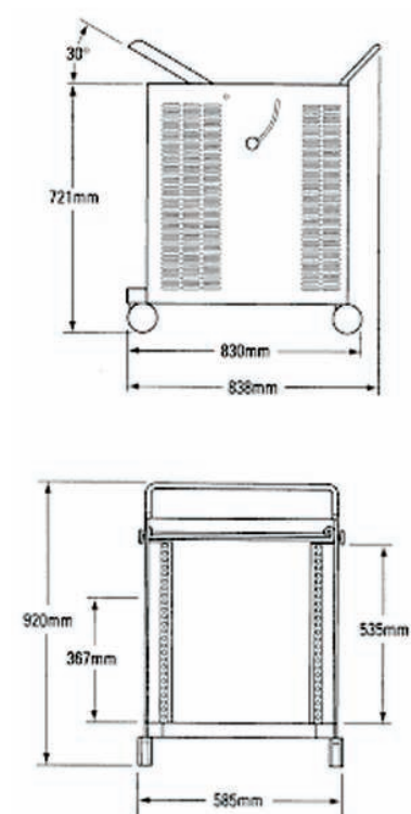
Figure 12. Agilent 1181BZ testmobile cart dimensions.
